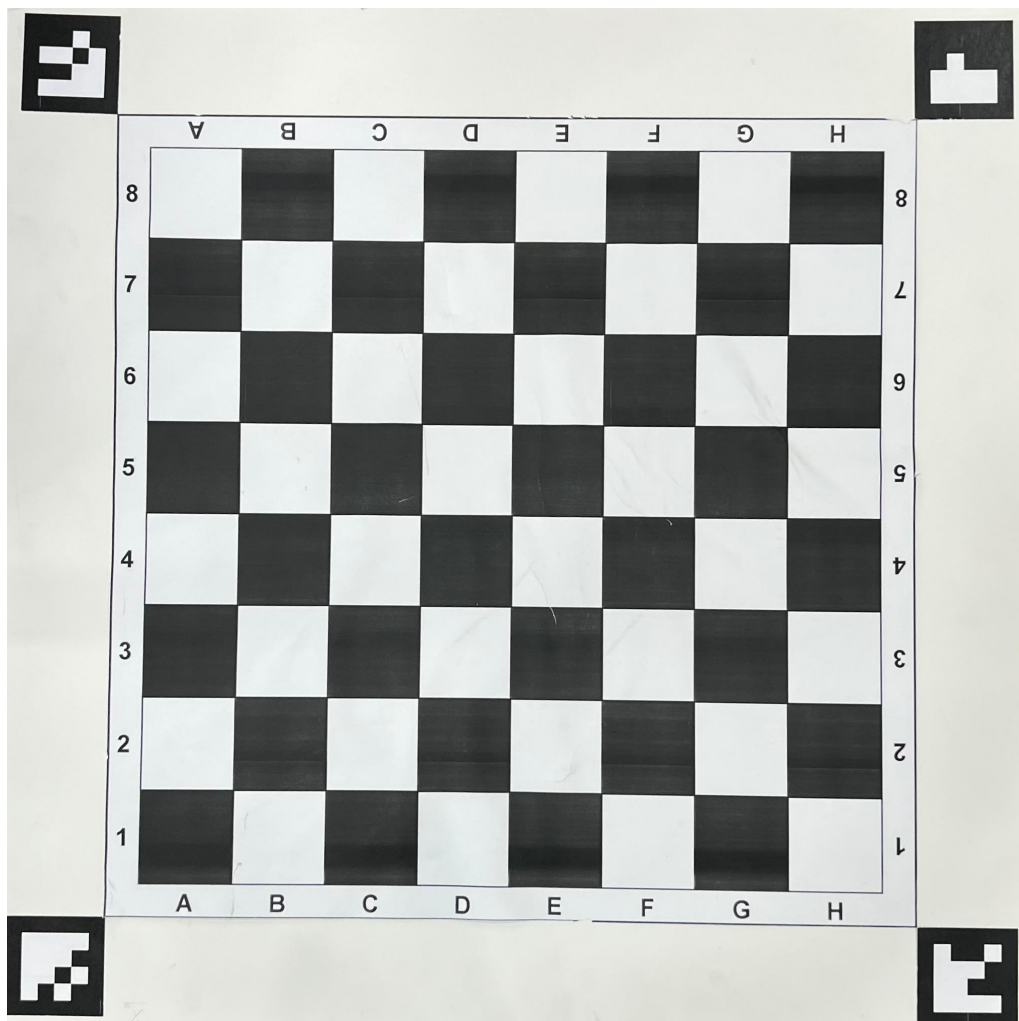
Figure 3.2: Chessboard setup with four ArUco markers used for camera-to-board calibration.
