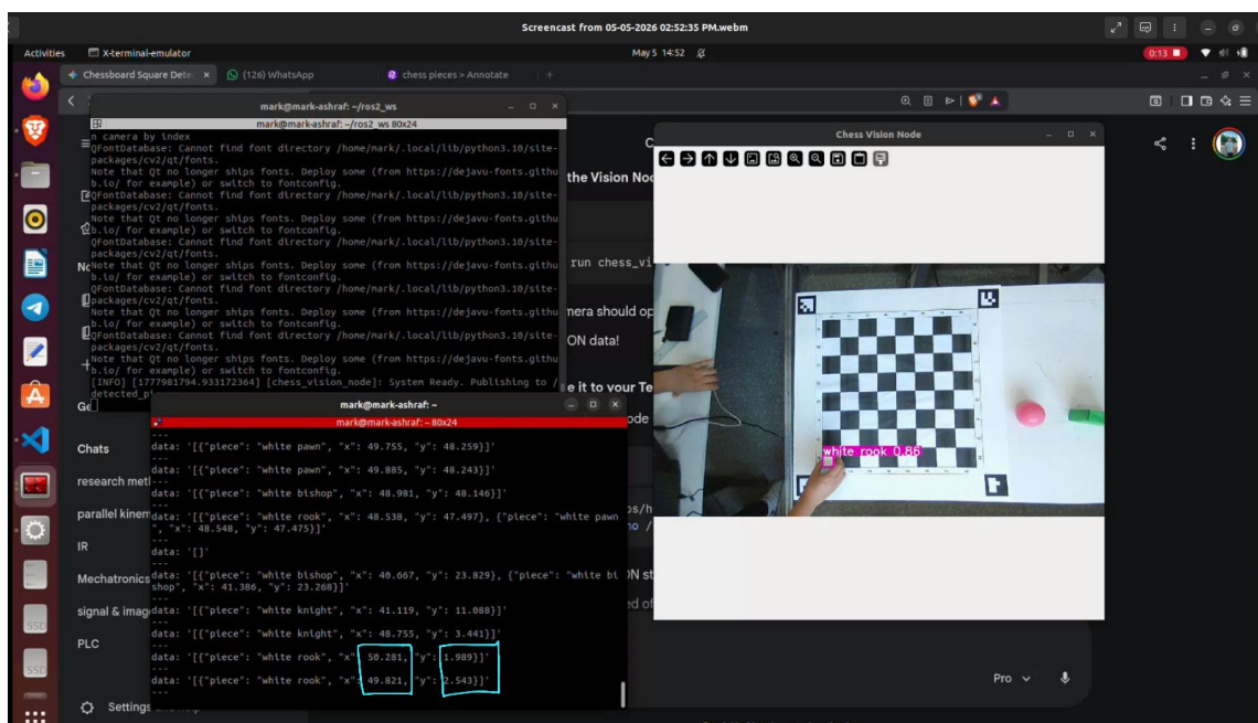
Figure 5.2: YOLO detection output showing detected chess pieces and their x,y positions.
