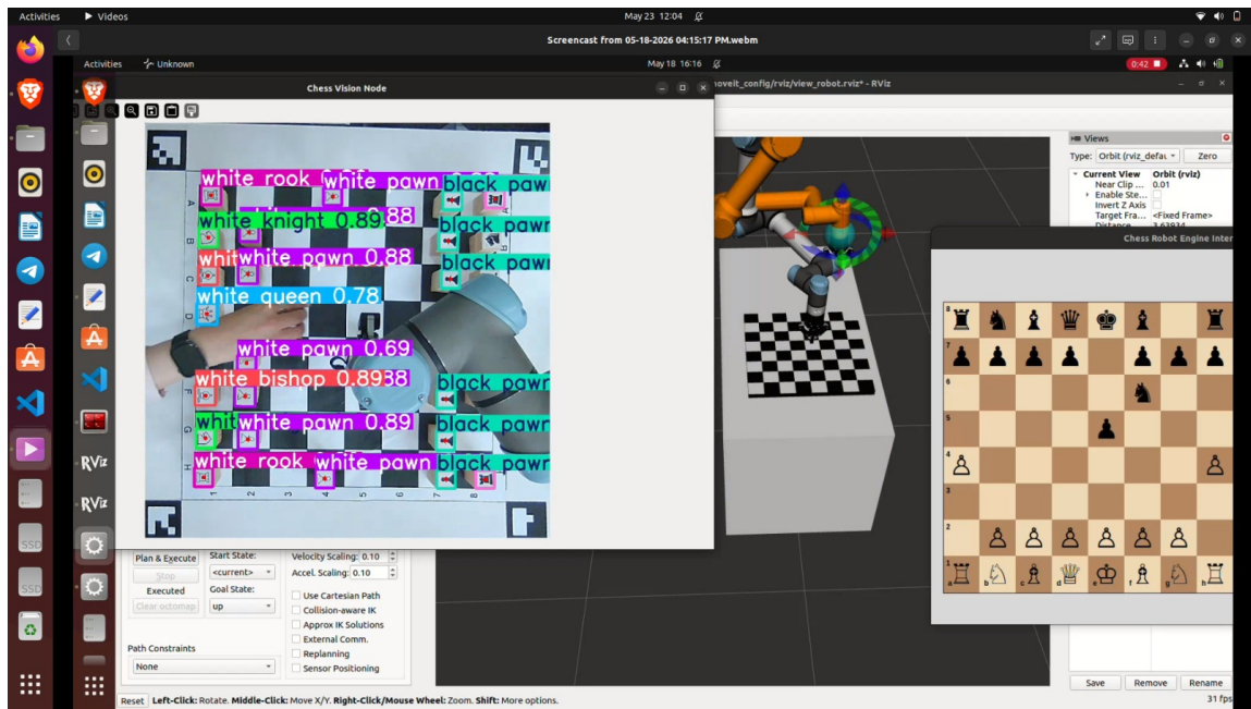
Figure 2.1: Combined system view showing YOLO detection, chess interface, and robot setup.
